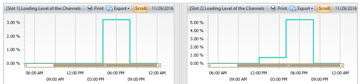
Figure 87: The loading level in the time slots of a MOTOTRBO IPSC system
