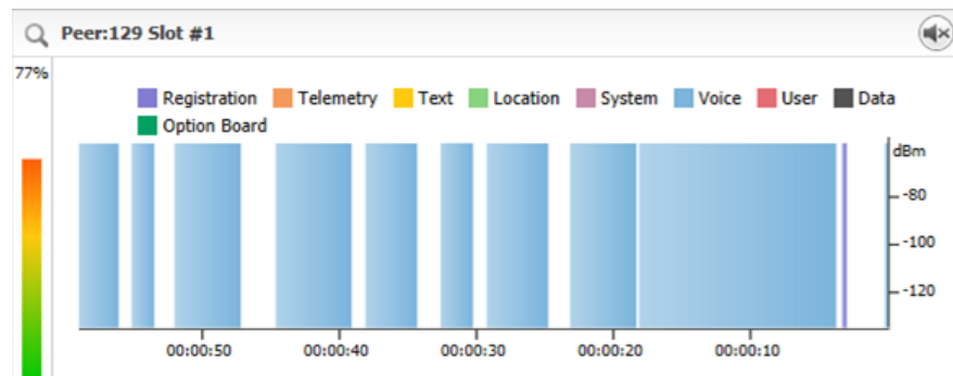
Figure 37: The real-time monitor displays traffic in the slot selected in the View pane
