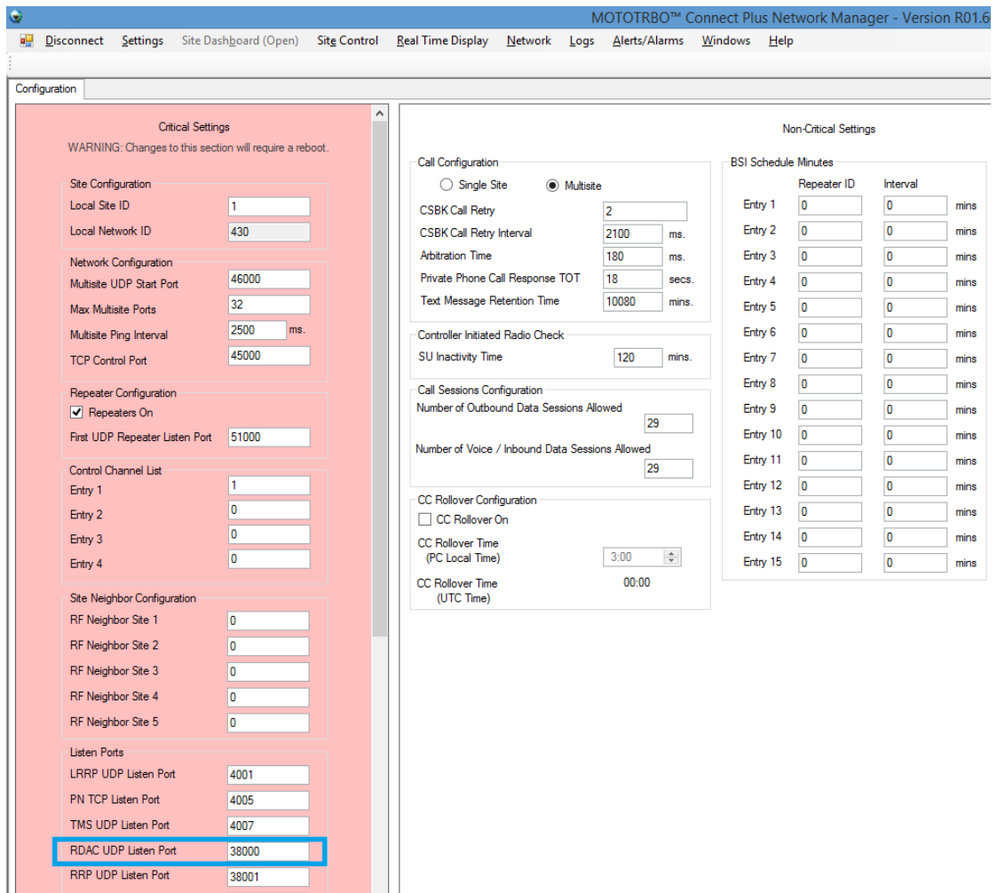
Figure 11: RDAC UDP Listen Port of the XRC controller
