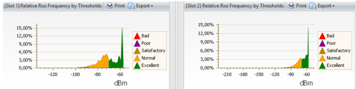
Figure 93: A MOTOTRBO IPSC system traffic ranged by RSSI level thresholds
