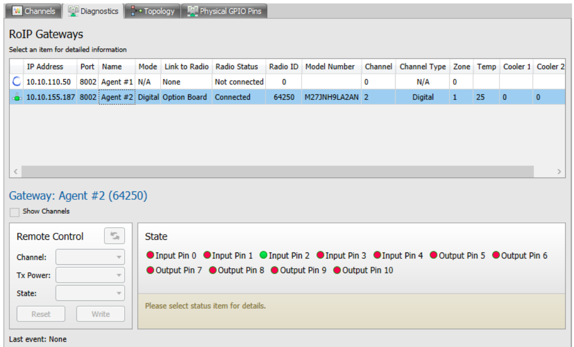
Figure 42: Diagnostic information for all RoIP gateways
