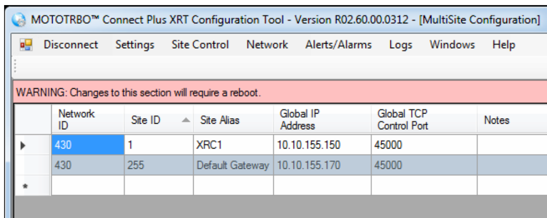
Figure 9: Connect Plus multi-site configuration tool
